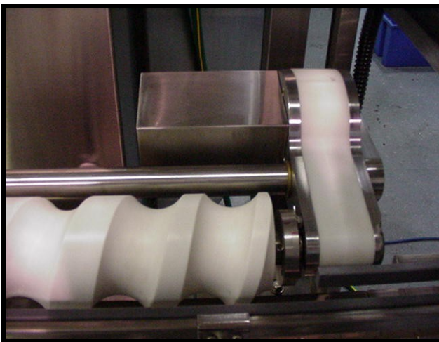
Interchangeable product timing screws
